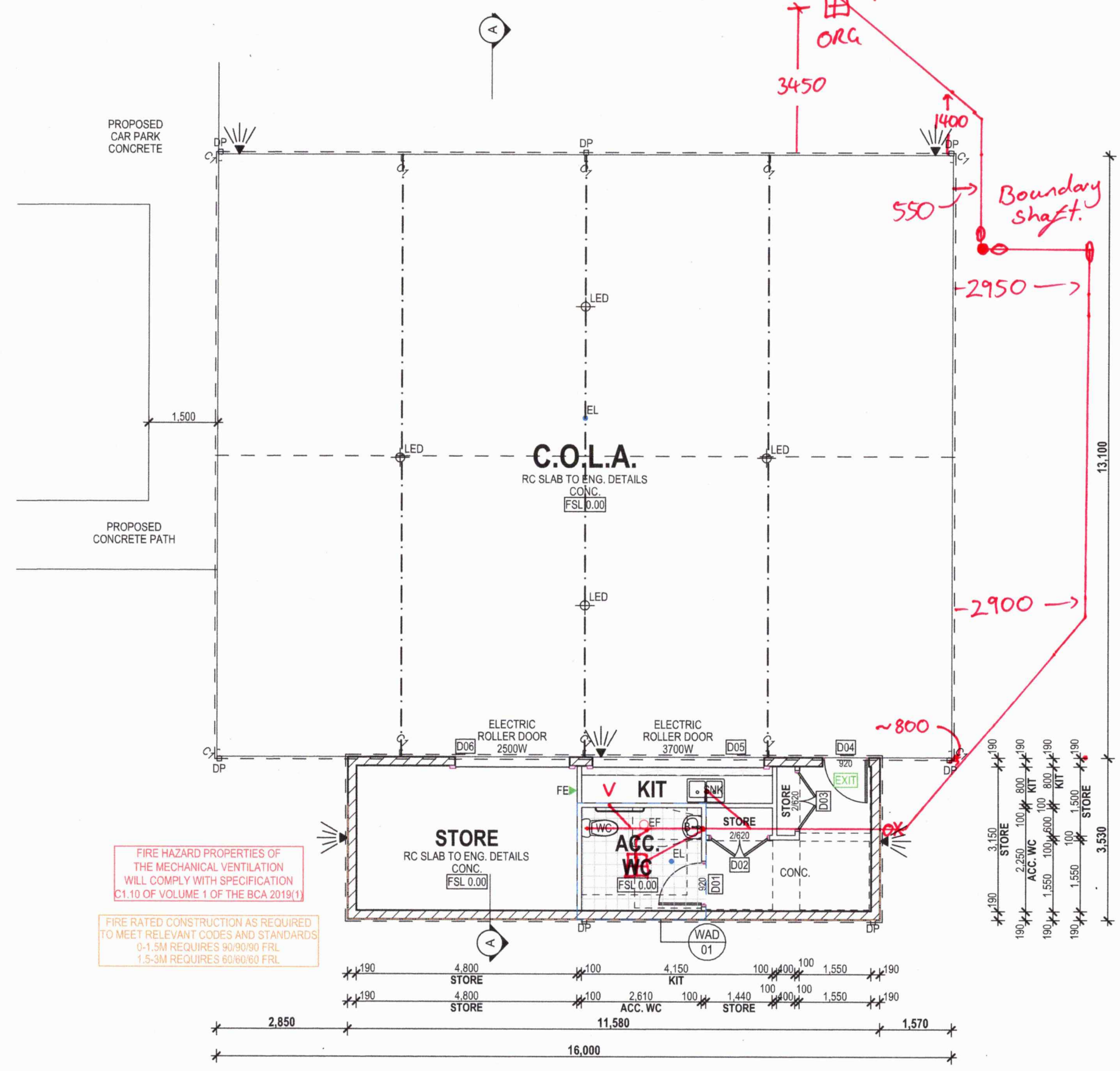
PROPOSED FLOOR PLAN SCALE 1:100@A3
